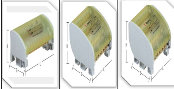
125 AMP. 7x12mm 7-30 D.2K.DAĞ. 80 AMP. 6,5x9mm 7-30 D.3K.DAĞ. 125 AMP. 7x12mm 7-30 D.3K.DAĞ.
