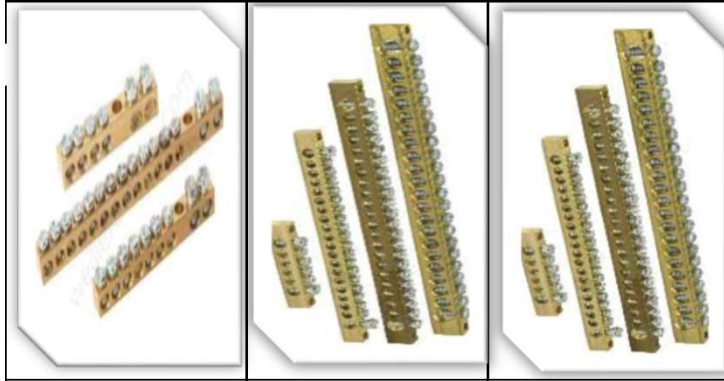
80 AMP. 6,5x9mm 4-22 DEL TOPRAK 80 AMP. 6,5x9mm 4-40 DEL TOPRAK 125 AMP. 7x12mm 4-40 DEL TOPRAK
